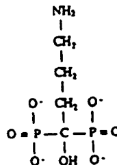
Alendronate
